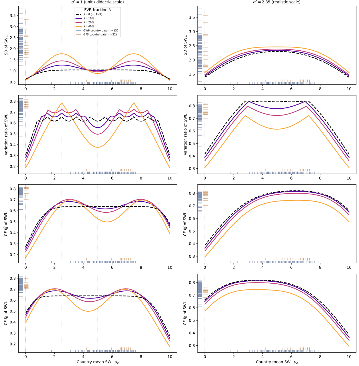
Figure 1: Analytic FVR bias curves for four dispersion statistics. Analytic FVR bias in four dispersion statistics as a function of the sample mean \mu , one curve per focal-responding share \lambda \in \{0, 0.1, 0.2, 0.4\} ; there is no sampling noise (Appendix S3.1). Rows: standard deviation; the ordinal variation ratio ( 1 - \max_k p_k , the share of responses not at the modal category); the Cowell–Flachaire downward-looking status index I_0^D ; and the Cowell–Flachaire upward-looking index I_0^U . Columns: the unit scale \sigma^* = 1 (left) and the realistic scale \sigma^* = 2.35 (right) — the latter the empirical mean within-country life satisfaction standard deviation across the GWP and GFS countries. In each panel the \lambda=0 curve is the bounded-scale (censoring) baseline; its vertical distance to the \lambda>0 curves is the FVR bias. Marginal rugs mark the real GWP+GFS country means (horizontal axis) and country dispersion values (vertical axis). The \lambda legend (top-left panel) is common to all eight panels.
