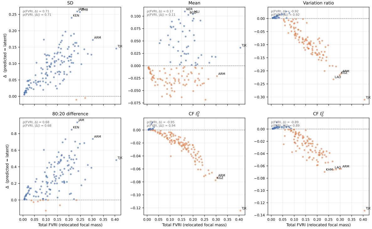
Figure S7.1: How much the FVR corrections cancel. Each panel plots, per country, the signed correction \Delta = \text{predicted} - \text{latent} for one statistic against the country's overall FVRI (total relocated focal mass), Gallup Cantril ladder. For the dispersion and ordinal statistics the correction grows nearly monotonically with the relocated mass (Spearman correlations annotated), whereas for the mean a large relocated mass yields almost no net correction: rounding toward 10 and toward 0 largely offset. Extreme countries are labelled.
